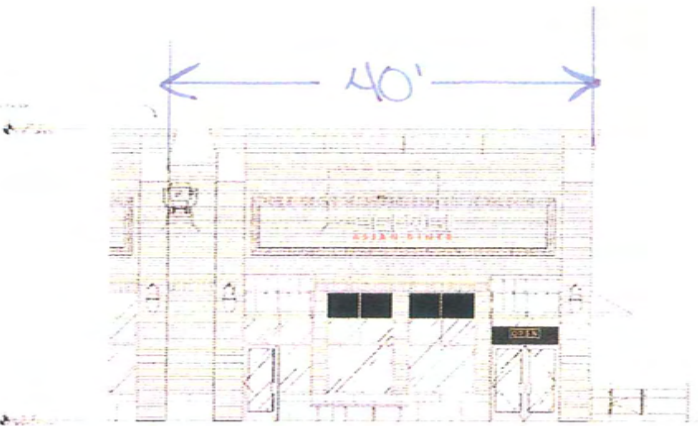
NORTH ELEVATION (NO ACTION REQUIRED) SCALE 3/32" = 1'-0"
