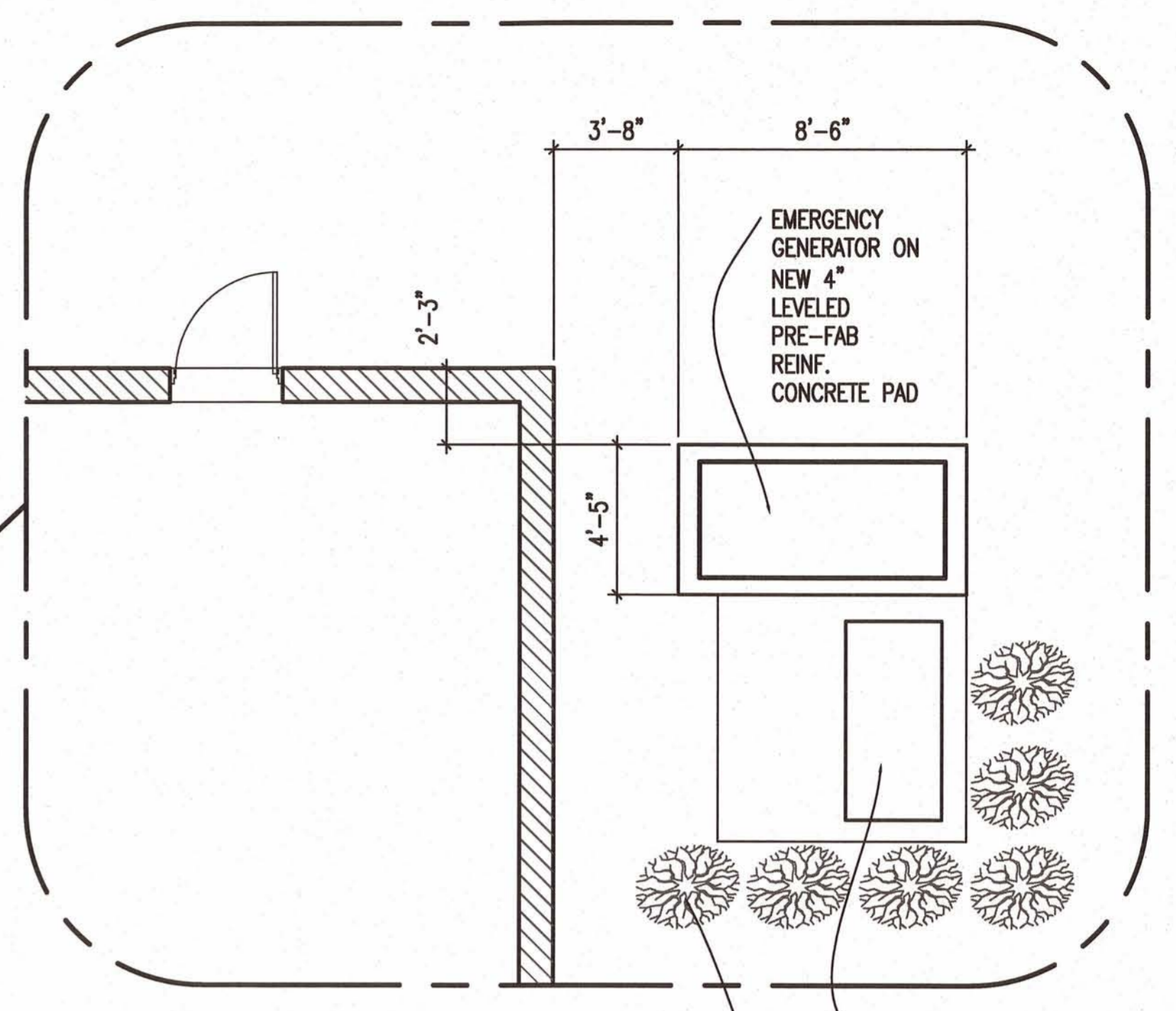
PARTIAL GROUND FLOOR PLAN SCALE: 1/4" = 1'-0"
