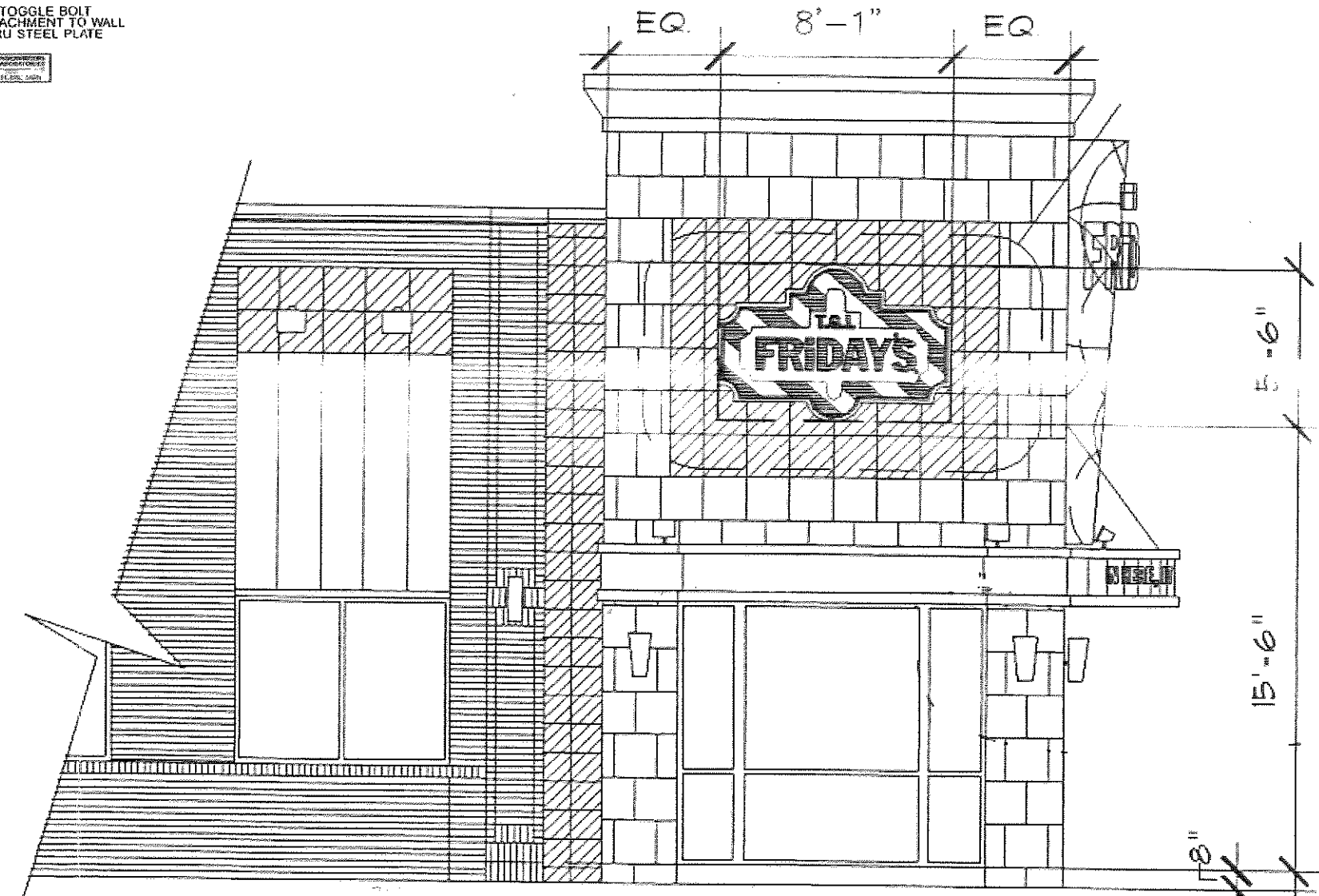
SIDE ELEVATION SCALE: 3/16" = 1'-0"
