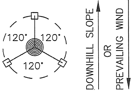
STAKING/GUYING LOCATION
